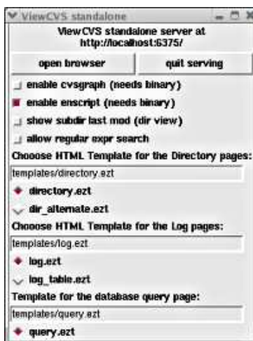
Figure 6: ViewCVS Configuration Dialog Box
