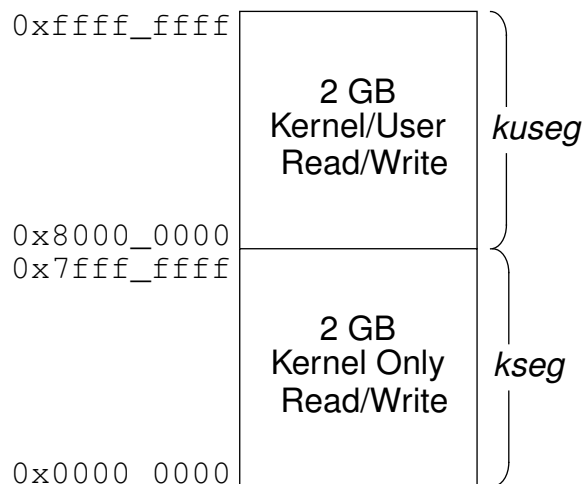
Figure 8: SMIPS virtual address space
