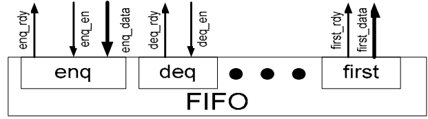
Figure 2: FIFO Interface
