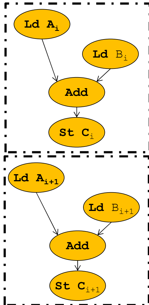
Scalar code
