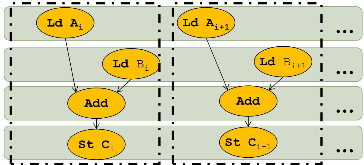
Vector code
